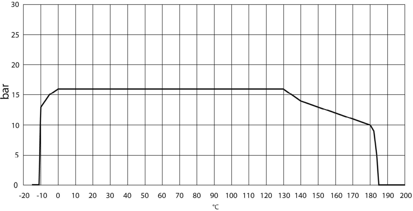
PRESSURE/TEMPERATURE DIAGRAM
